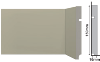
496 RP Cinza Glacial Skirting Board Glacial Gray Zócalo Gris Glacial
