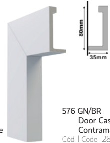
553 GN/BR Door Case White - Adjustable Contramarco Blanco - Ajustable Cód. | Code - 28369
